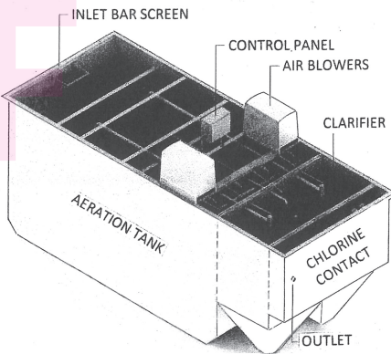
TYPICAL 15,000 GPD UNIT
